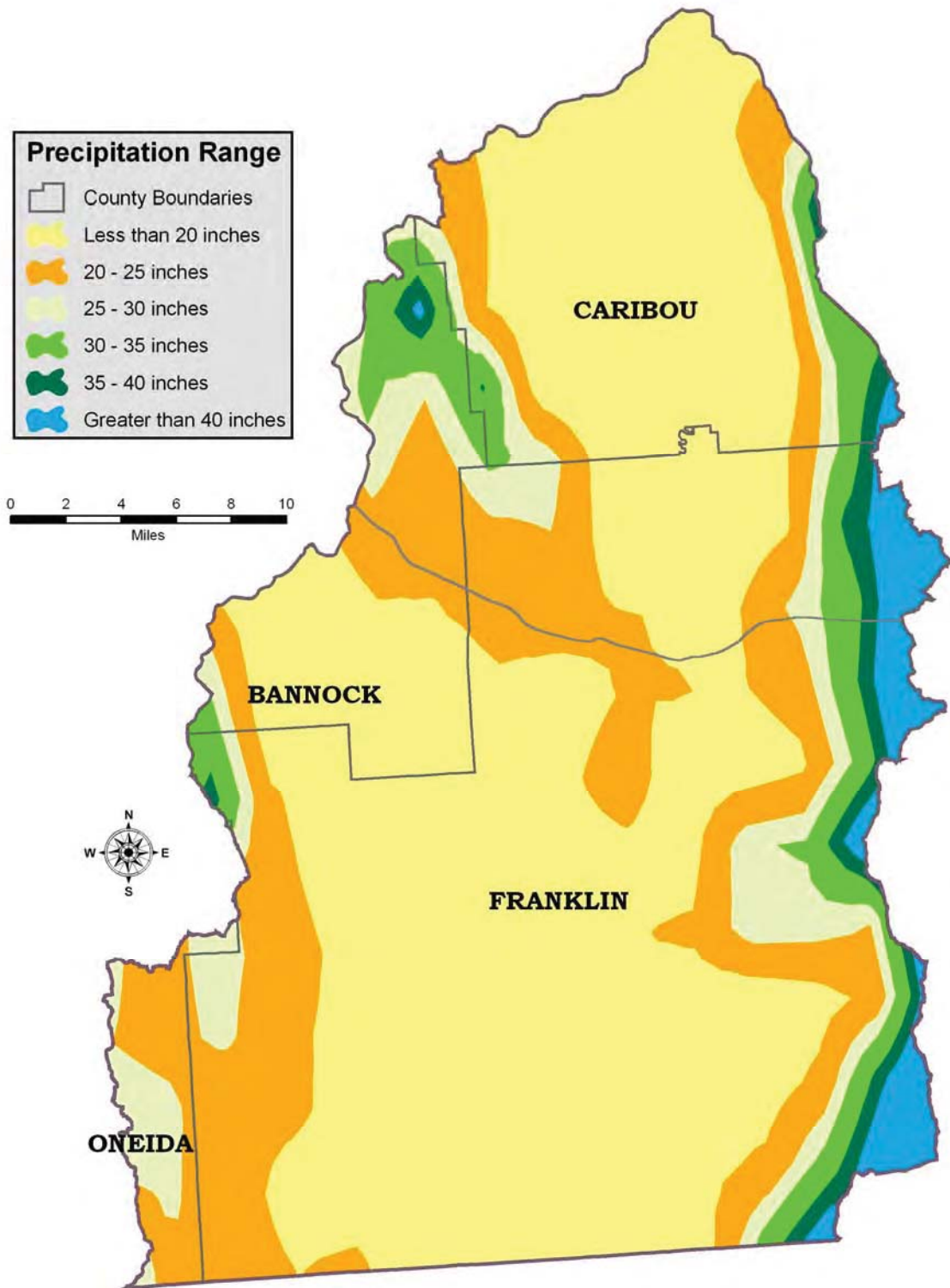
Figure 3. Precipitation in the Southern Middle Bear Subbasin
